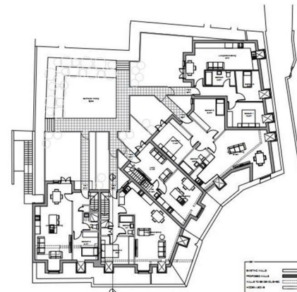
3 Proposed Site Plan 1:100
