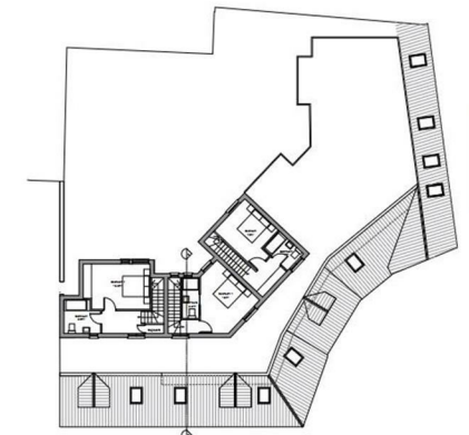
4 Proposed Layout Plan 1:100
